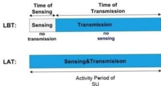
Figure 2. The two main functioning modes of SU activity. Listen-before talking the sensing period and no sensing is performed during the LAT): sensing and transmission are made concurrently.
