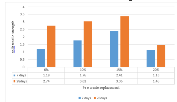
Fig. 3.2. Average split tensile strength for M20 grade of concrete
