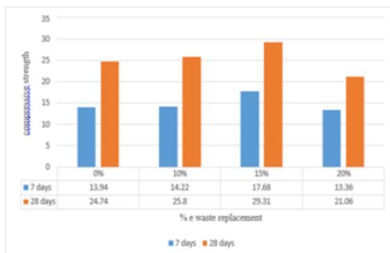
Fig. 3.1. Average compressive strength for M20 grade of concrete
