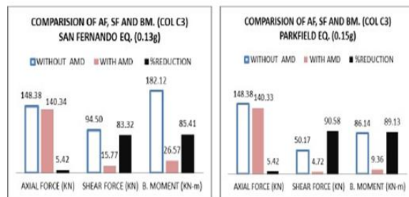
Fig. 5.11 Axial force, SF and Fig.5.12 Axial force, SF, BMB for single AMD, for single AMD, for San Fernando Earthquake for Parkfield Earthquake
