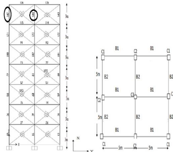
Fig. 5.1 Plan and Elevation of building with dampers
