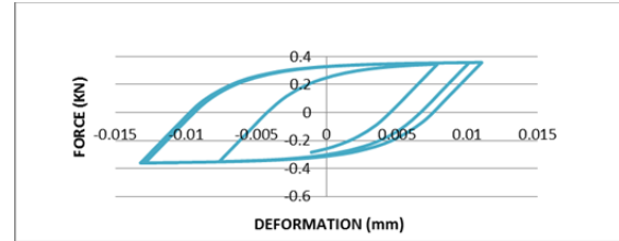
Fig. 4.3 Typical hysteresis loop of metallic damper
