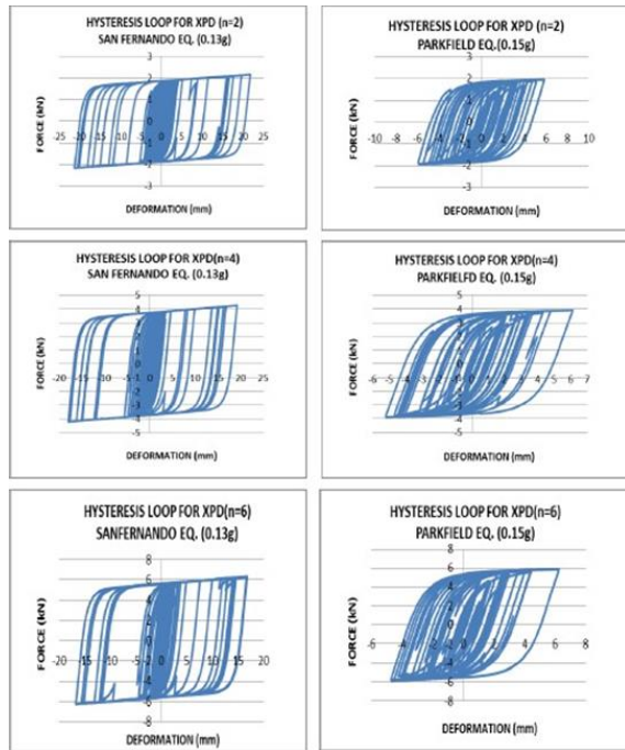
Fig. 5.6 Hysteresis loop for Fig. Hysteresis loop for San Fernando earthquake parkfield earthquake
