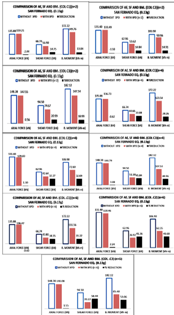
Fig. 5.4 Axial force, shear force and bending moment for XPD (n=2, 4 and 6) for column C1, C2 and C3 at top story of building for San Fernando earthquake
