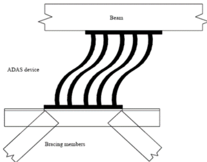
Fig.1.3b Typical metallic plate damper installation and ADAS devices deformation
