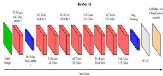
Figure 1. ResNet-18 Architecture
