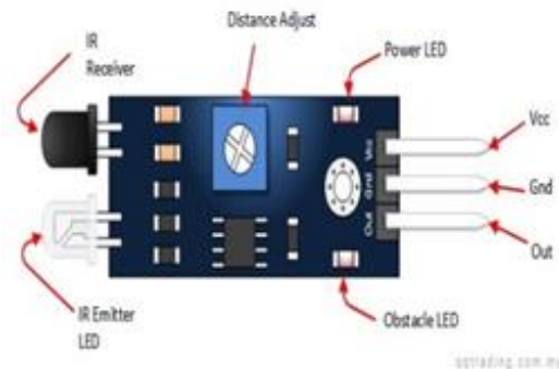
Fig.4. Infrared Sensor
