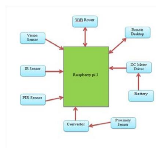
Fig.1. Block diagram of the entire system
