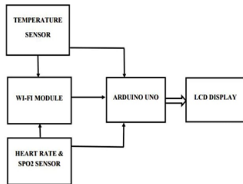
Fig 1: Block Diagram of Patient Health Monitoring with an Arduino Based Smart Mirror
