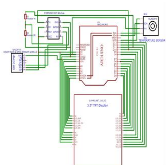
Fig 2. : Circuit Diagram of Patient Health Monitoring with an Arduino Based Smart Mirror
