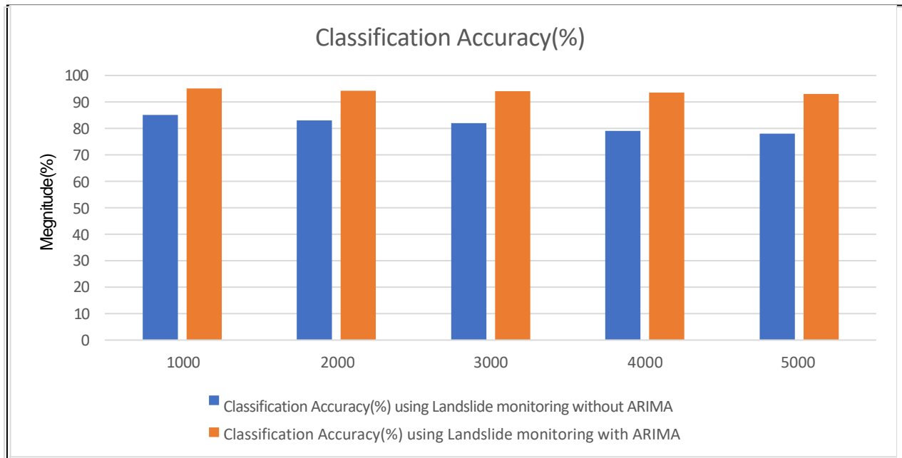
Figure 2: Visualization result corresponding to classification accuracy
