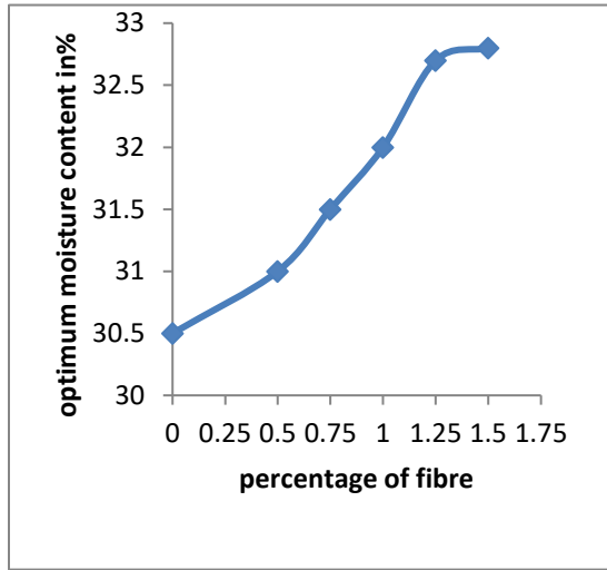
Fig 3. Variation in optimum moisture content
