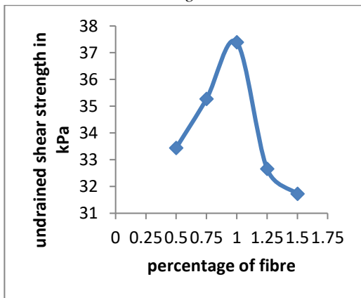
Fig 4. Shear strength of clay by inclusion of Coir fibre
