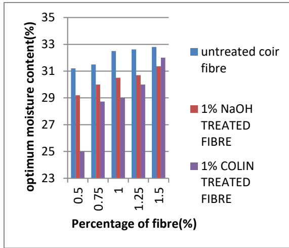
Fig 8. Variation in optimum moisture content of clay by inclusion of 1% sodium hydroxide treated fibre and 1% Dust cleaning reagent treated fibre. The optimum moisture content was higher for untreated fibre than treated fibre due to the presence of hemicellulose in coir fibre and washed away by treatment.
