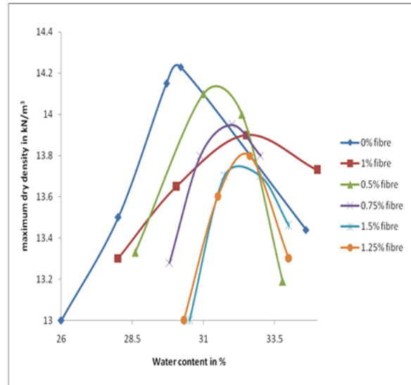
Fig 1. Compaction curves by inclusion of untreated fibres
