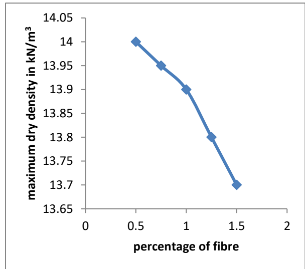
Fig 2. Variation of maximum dry density of clay by addition of coir fibre
