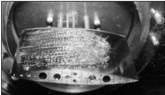
Fig. 5. Attached cavitation.
