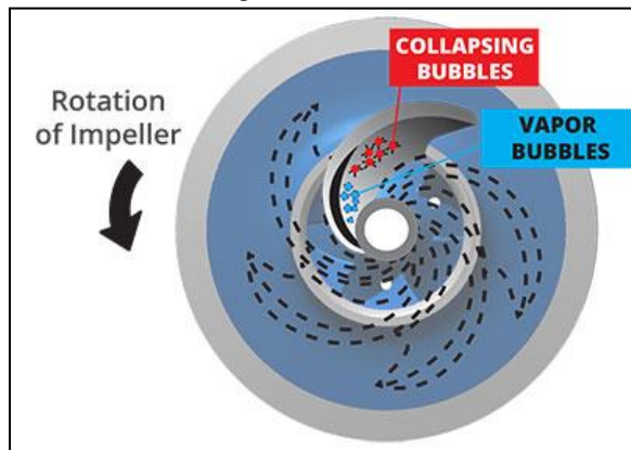
Fig. 2. Formation and collapsing of vapor bubbles. Some of situations where cavitation phenomenon is more likely to occur in the fluid flow through centrifugal pump.
