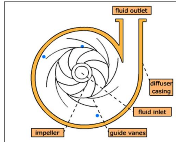
Fig. 1. Constructional features of centrifugal pump. The vanes are usually slope backwards, away from the direction of rotation. The blades of the rotating impeller transfer energy to the fluid & thus increase velocity. The fluid is sucked into the impeller through impeller eye and flows through the impeller channels formed by the curved blades between the shroud and hub. The fluid is accelerated by pulse transmission while following through the curvature of the impeller vanes from the impeller Centre (eye) outwards. It reaches its maximum velocity at impeller’s outer diameter and leaves the impeller into a diffuser or volute chamber [7-8].
