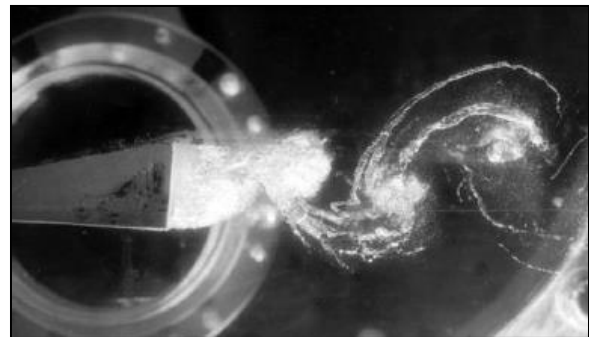
Fig. 7. Shear cavitation.
