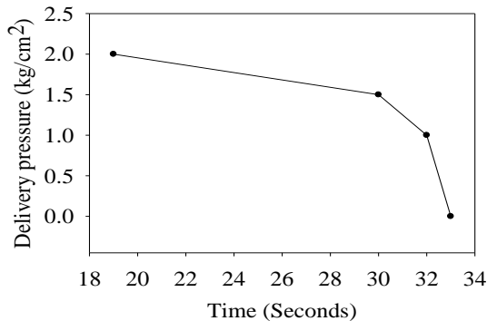
Fig. 3. Variation in delivery pressure with time.
