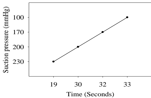
Fig. 2. Variation in suction pressure with time.
