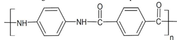
Fig.2 Aramid fibre structure
