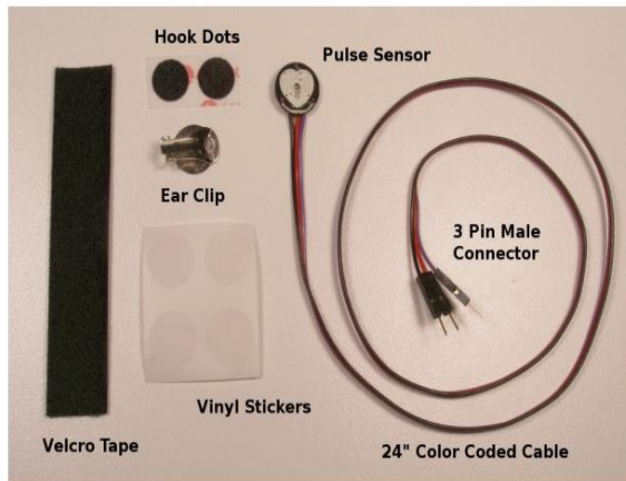
Fig: - Pulse Rate Sensor Kit
