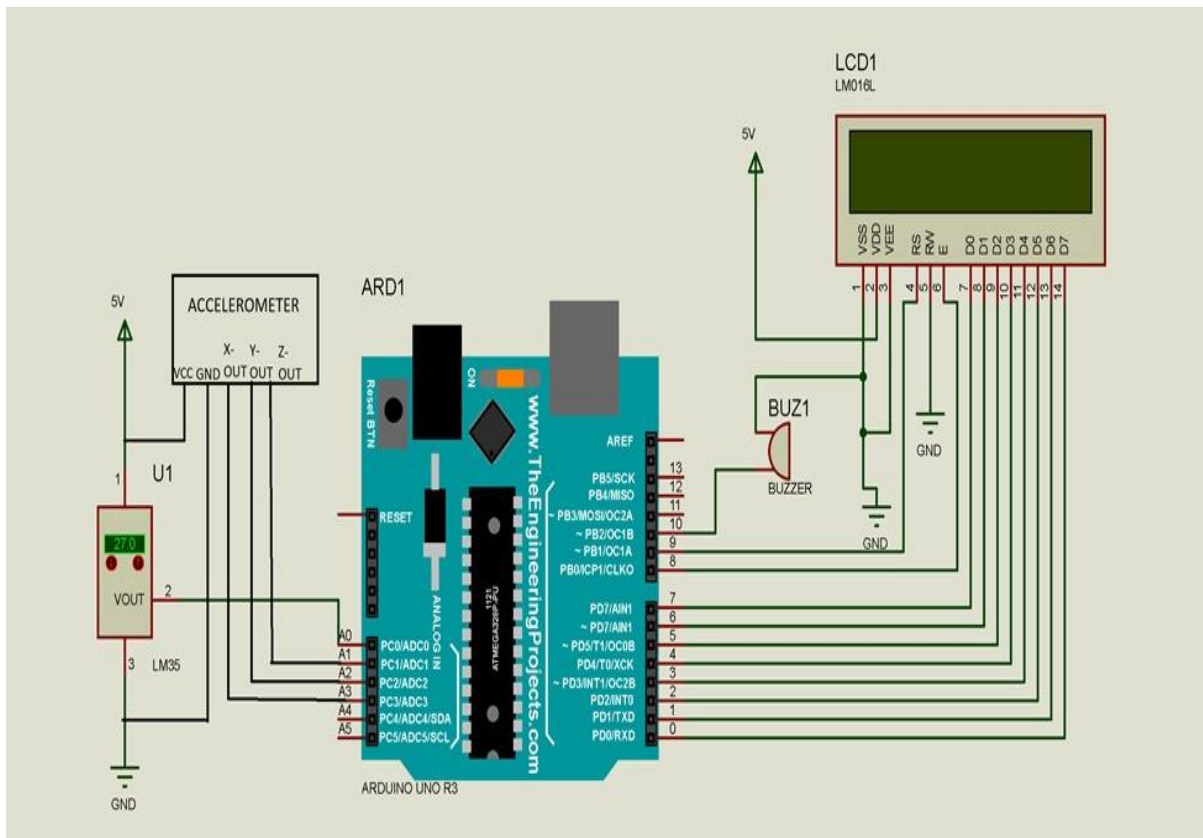
Fig - Circuit Diagram of System
