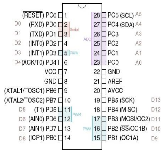
Fig: - Pin diagram of Atmega328 microcontroller
