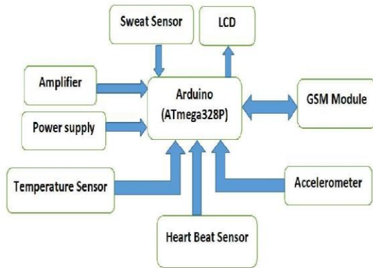
Fig: - System Block Diagram
