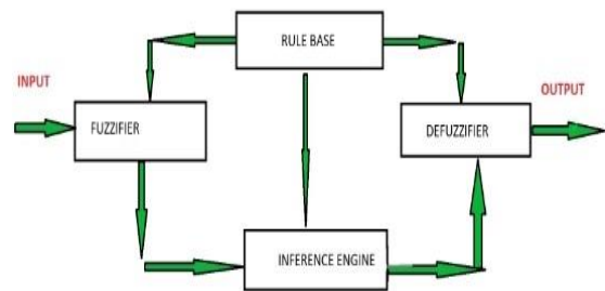
Figure 1.Fuzzy Logic Architecture[7]
