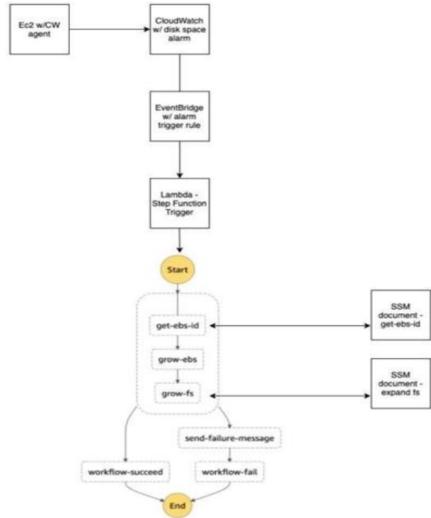
Fig 9. Architectural Flow chart –analysis of the design
