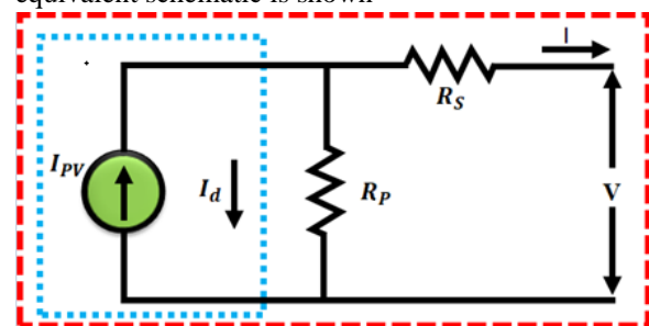
Fig. 2. PV System
