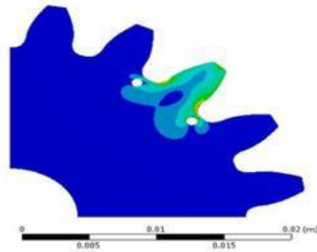
Fig.1.Equivalent stress maximum for diameter 8 mm
