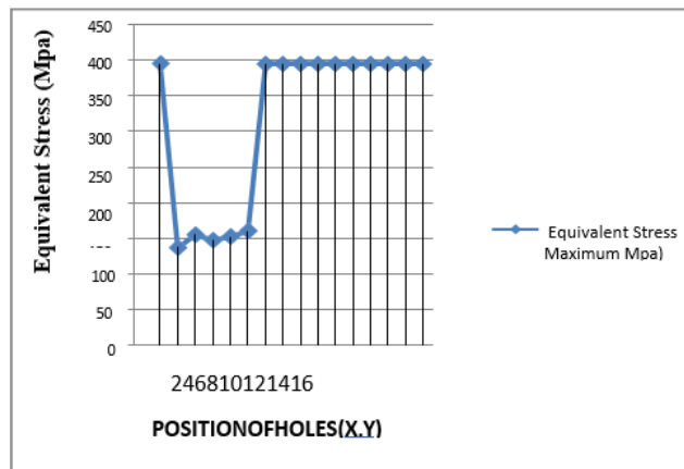
Fig5 Position of hole Vs Equivalent Stress Max
