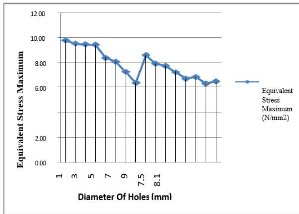
Fig4 Diameter of hole Vs Equivalent Stress Maximum
