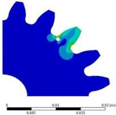
Fig.2 Equivalent stress maximum for location X=9.39 mm and Y= 13.86 mm
