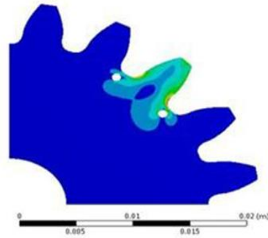
Fig. 3. Equivalent stress maximum for diameter 8 mm with 2 holes
