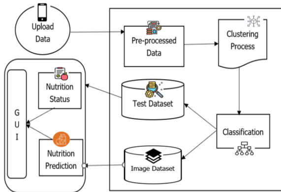
Figure 1: Architecture of the System
