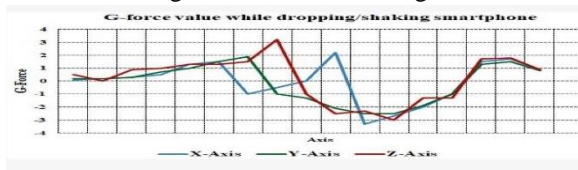
Fig 9: Experimental Graph
