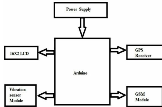
Fig 1: Arduino System
