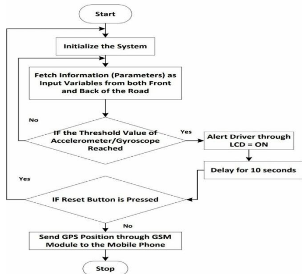
Fig 3: Accident detection alert System
