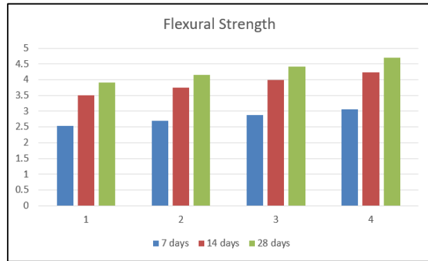
Graph 4 Flexural Strength
