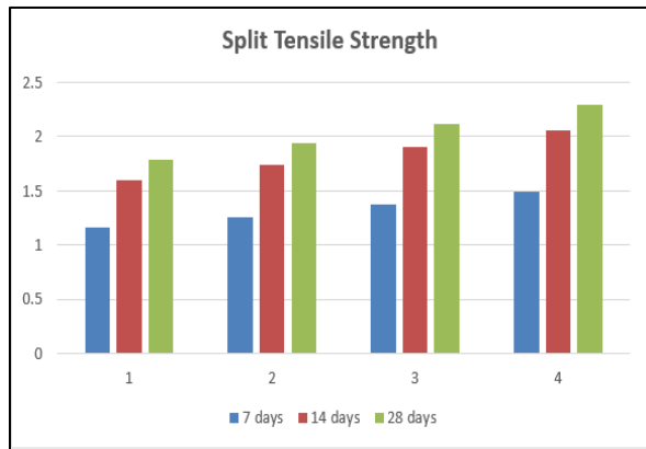
Graph 3 Split Tensile Strength
