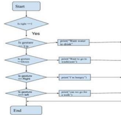
Fig. 4. Flowchart Software Implementation
