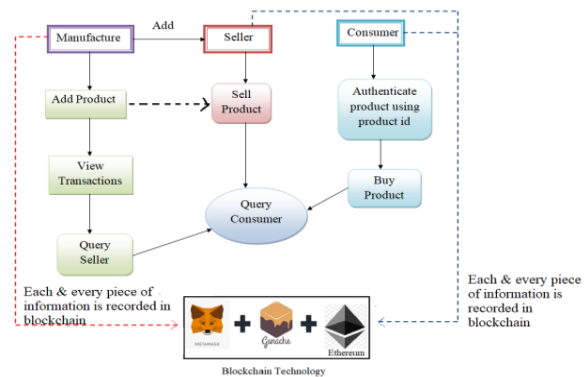
Fig 1 Proposed Architecture
