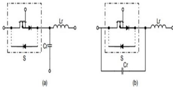
Figure 1. Zero-voltage (ZV) resonant switch
