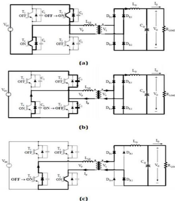
Fig. 4. Experimental circuit of the bidirectional DC- DC converter test
