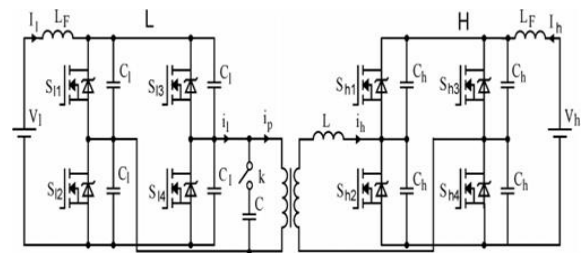
Fig.2(b). Proposed bidirectional DC-DC converter topology
