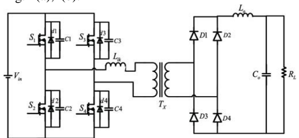
Fig.2(a). Full Bridge Phase Shifted Converter
