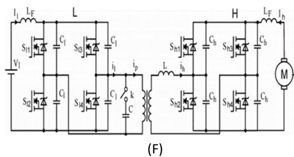
Fig. 4. Experimental circuit of the bidirectional DC- DC converter test
