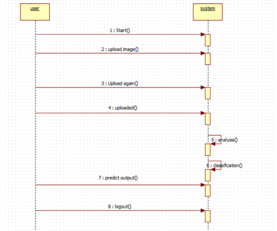
CLASS DIAGRAM:
