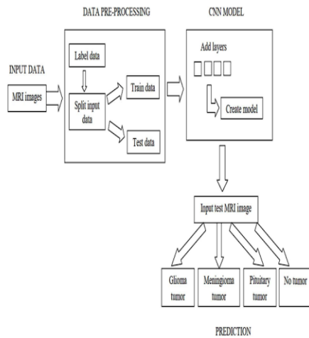
FIG 4.1 SYSTEM ARCHITECTURE
