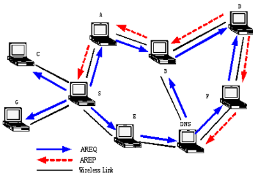
Figure 2 The secure DAD procedure to detect duplicate IP addresses and domain names
