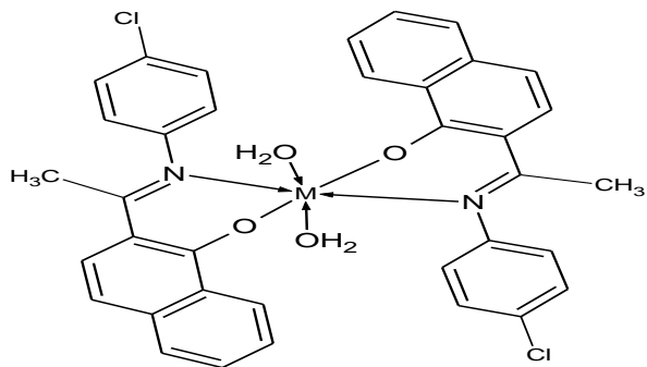
Figure 3. The metal-ligand binary binding proposed structure.
