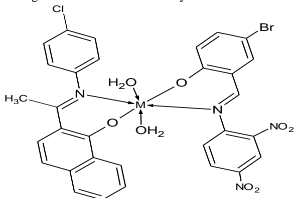
Figure 4. The metal-ligand ternary binding proposed structure.
