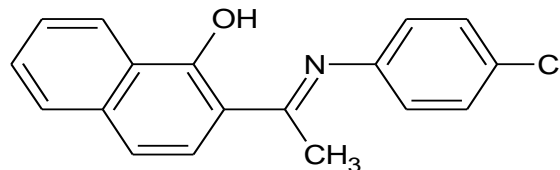
Figure 2. Secondary ligand 2-[(1E)-N-(4-chlorophenyl) ethanimidoyl] naphthalen-1-ol
