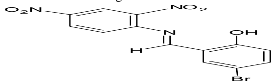
Figure 1. Primary ligand 4-bromo-2-[(E)-[(2,4-dinitrophenyl) imino] methyl] phenol
