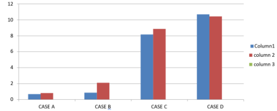
CBR RESULTLS for CASE A,B,C& DFOR 2.5mm&5mm penetration.
