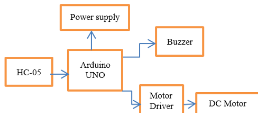
Fig 3.1 Block diagram of stable part of the system
