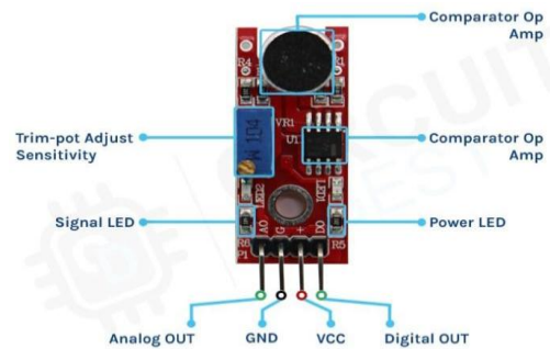
Fig 4.6 Sound Sensor
