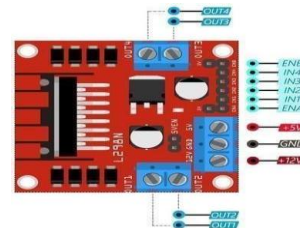
Fig 4.2 Motor driver
