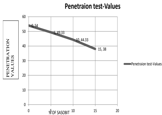
Graph 1: Penetration values vs % of sasobit
