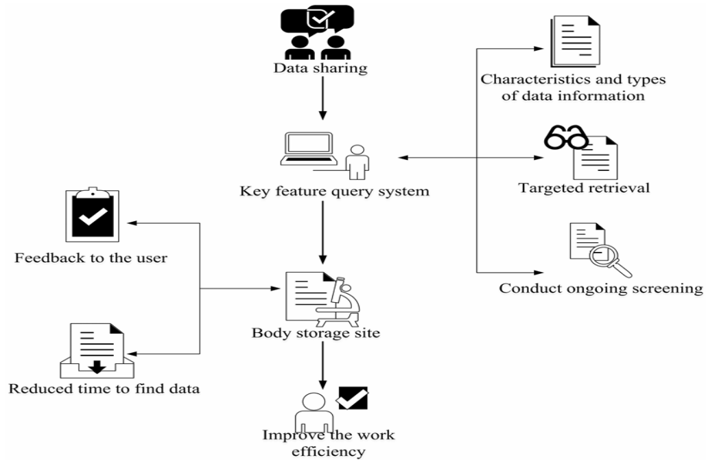
Figure 2: Data-sharing analysis.
