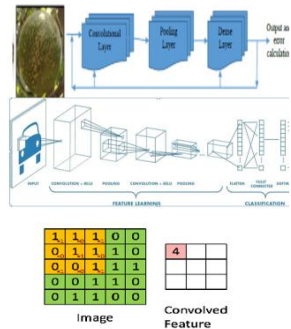
Figure-2: CNN Architecture
