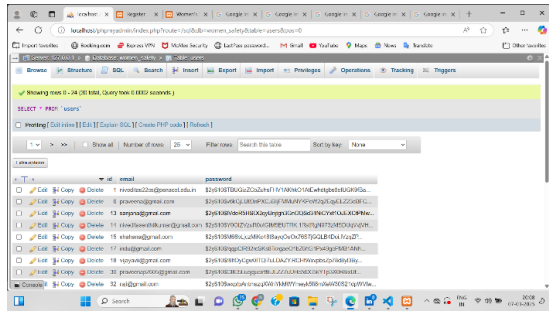
Figure 4: Database Connectivity.
