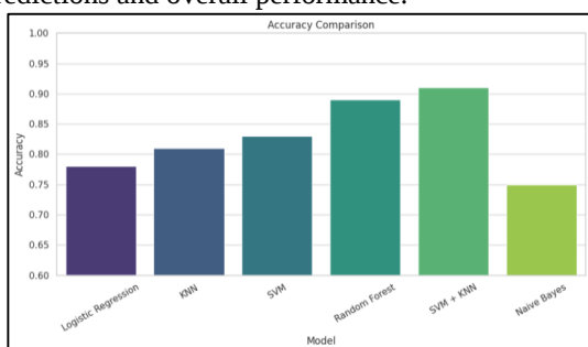
Figure 2: Accuracy Comparison of different ML Models
