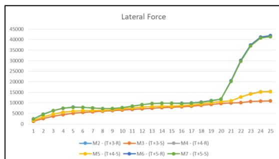
Graph 4 Lateral Force
