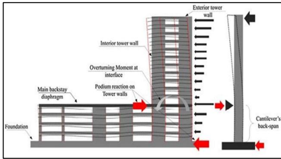
Fig 1 Tower with Podium
