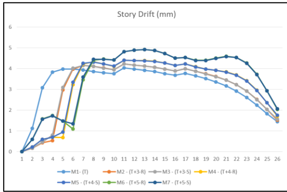
Graph 3 Story Drift (mm)
