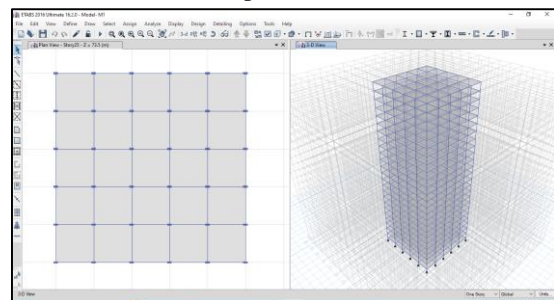
Fig 2- M1. Tower without podium (T)
