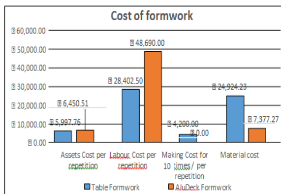
Fig. 4. cost and time comparison of Table and AluDeck type of formwork systems
