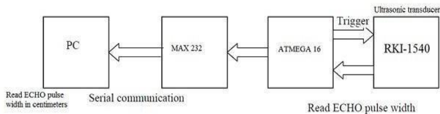
Figure 4.2: Block diagram of the system
