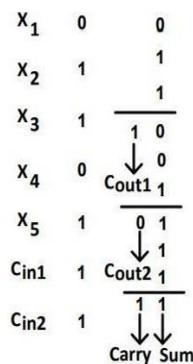
Figure 4.1: 5:2 Compressor Example
