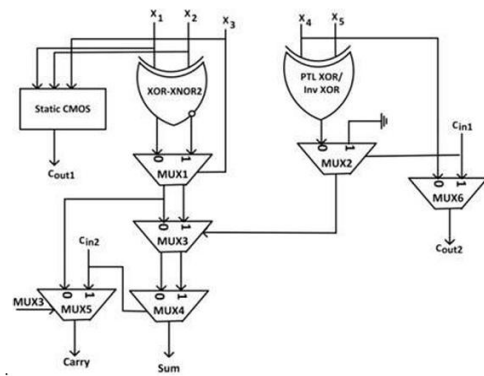
Figure 4.2 Inexact 5:2 Compressor using Probabilistic Pruning
