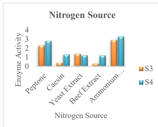
Fig 6: Effect of Nitrogen Source
