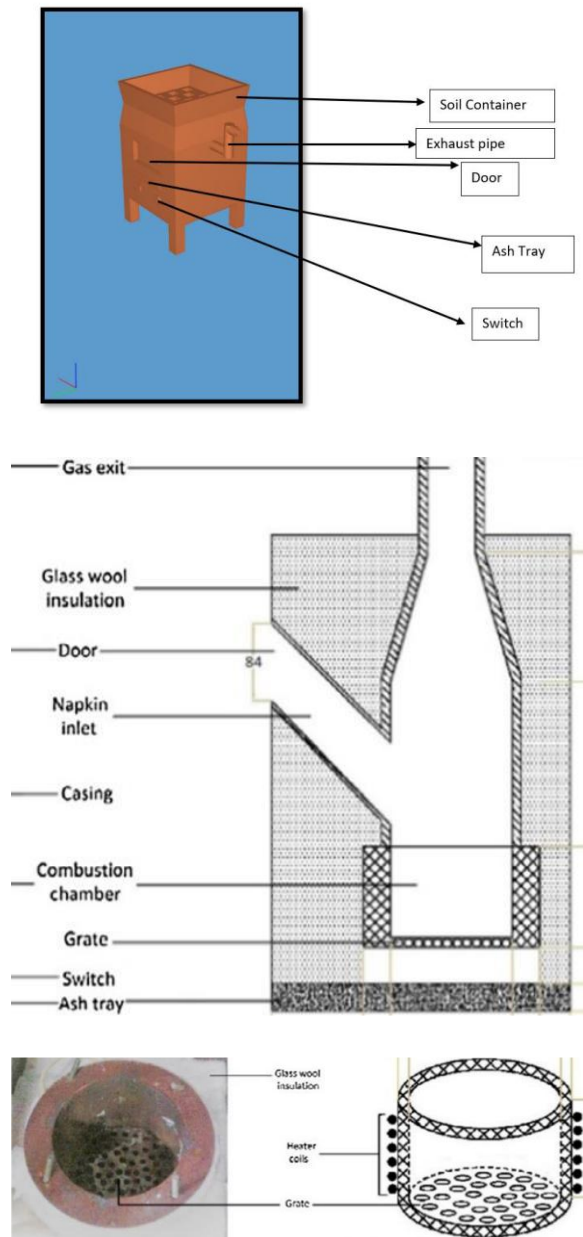
Fig 4.1: Design of Incinerator
