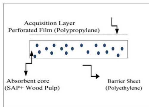
Fig 3.1: Layers of sanitary napkin
