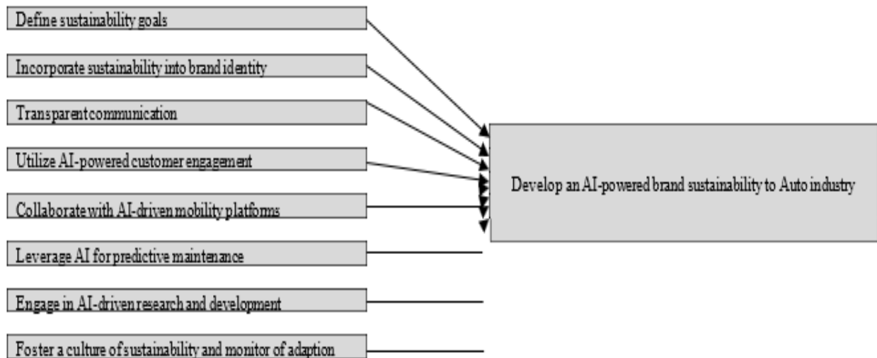
Fig. 1. Hypothesis model
