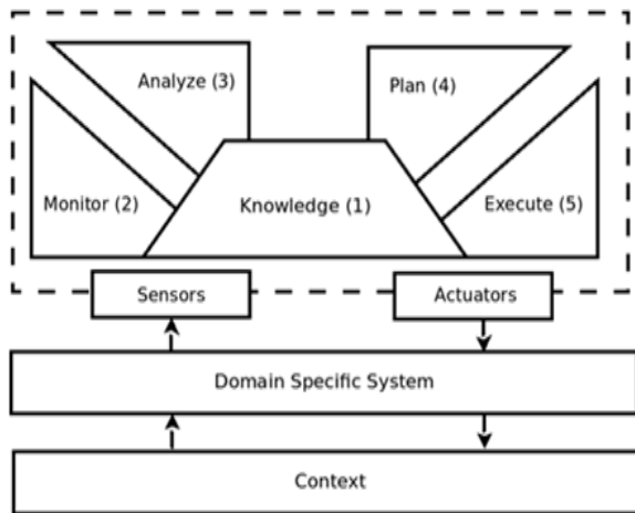
Fig.3.The MAPE-K model[10]
