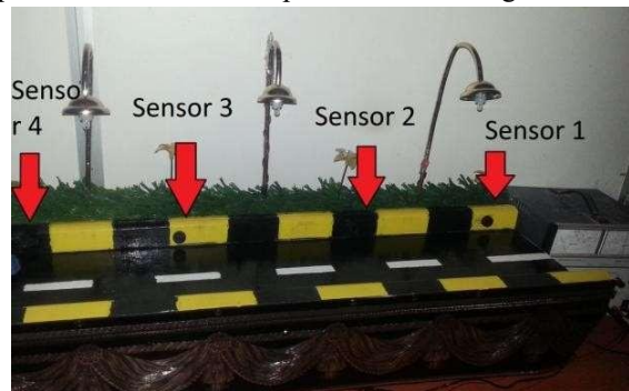
Fig.9 Prototype of street light system
