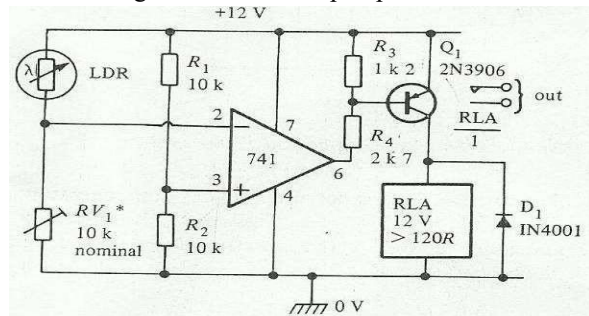
Fig. 7 LDR circuit
