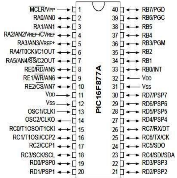
Fig. 6 Pin diagram of PIC16F877A microcontroller
