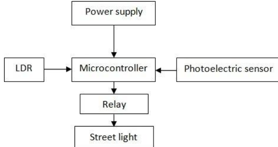
Fig. 1 Block diagram of street light system
