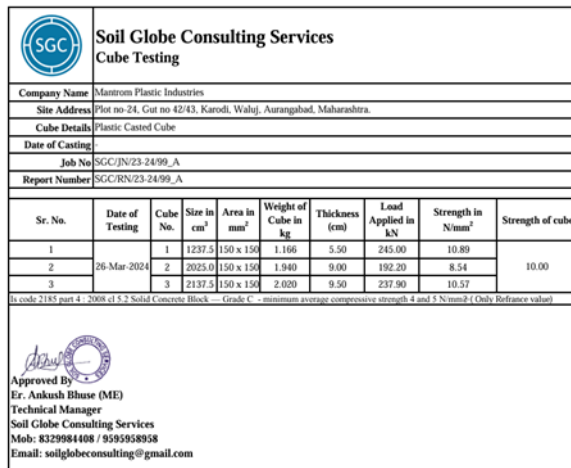
Fig. 2. Certified compressive strength test report of plastic-based block (Soil Globe Consulting Services).
