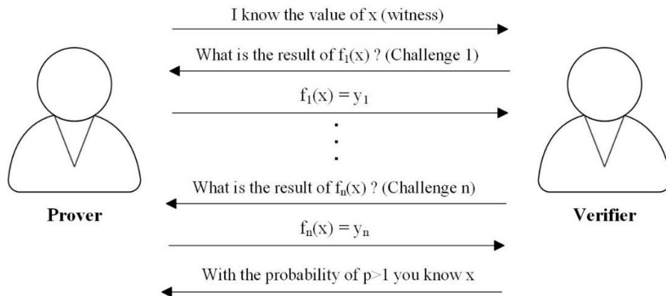
Fig. 7. Outline of a typical ZKP protocol
