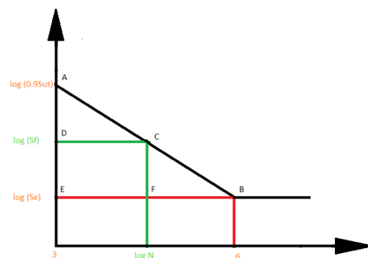
Fig. 2 S- N Diagram
