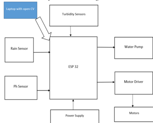
Figure 1. Block Diagram of Techno Dam
