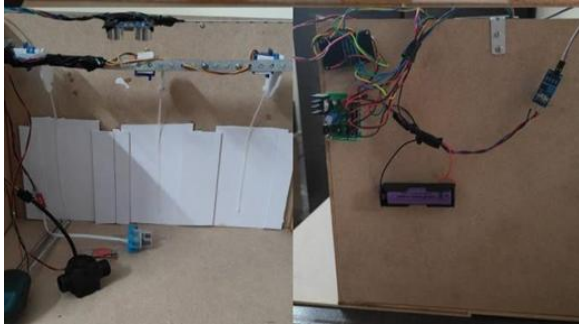
Figure 3. Hardware Model Implementation
