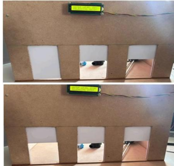
Figure 5: Automated Dam Gate Control
