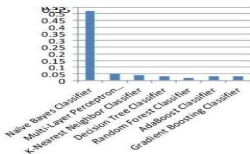
Fig. 7. Comparison of MSE for all specified supervised machine learning model
