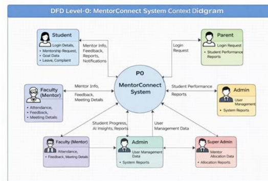
Fig. 5. Data Flow Diagram (Level-0)
