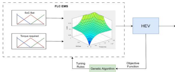
Figure 4. Optimal FLC EMS redrawn from [75].
