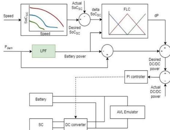
Figure 8. FLC combined with LPF proposed by [101].
