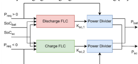
Figure 6. Adaptive FLC EMS: powering-braking-based [87].
