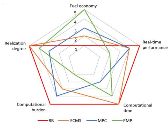
Figure 2. EMS performance comparison redrawn from [35].
