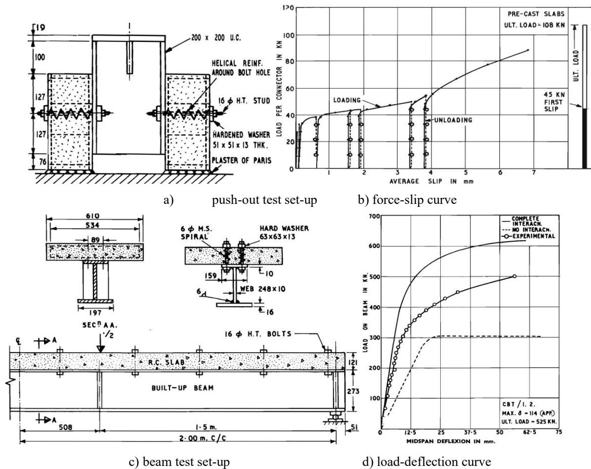
Fig. 2.2 Friction-grip bolts push-out and beam tests [Marshall et al, 1971].
