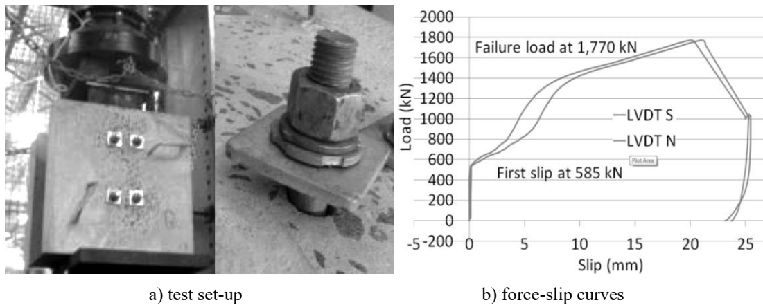
Fig. 2.4 Friction grip bolts [Lee and Bradford, 2013].
