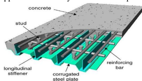
Fig- 1.1 Steel-concrete composite deck
