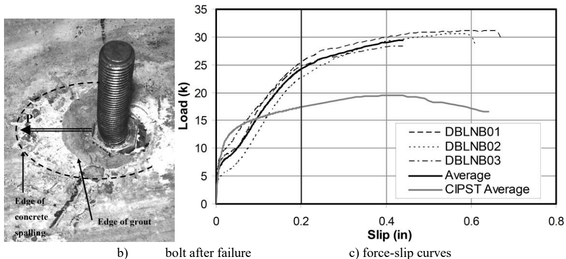
Fig. 2.9 Double-nut bolt (DBLNB) shear connector [Schaap, 2004].
