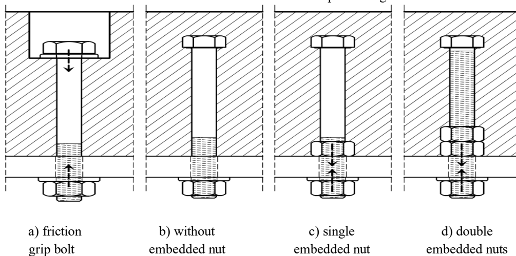
Fig. 1.3 Bolted shear connectors types.
