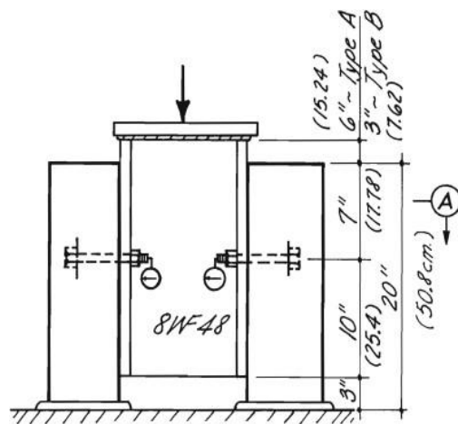
a) test set-up
