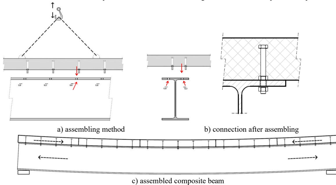
Fig. 1.2 Prefabrication with use of casted bolted shear connectors.
