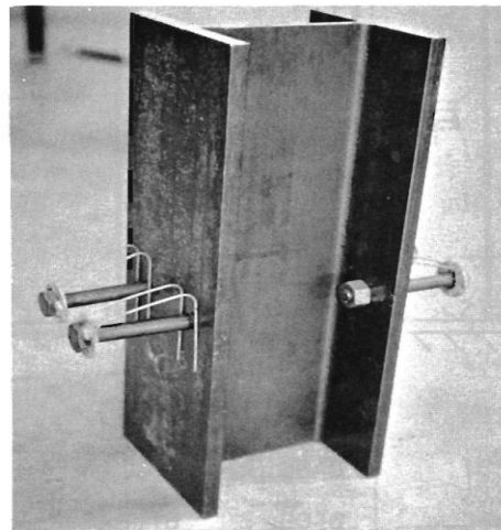
b) bolt installation
