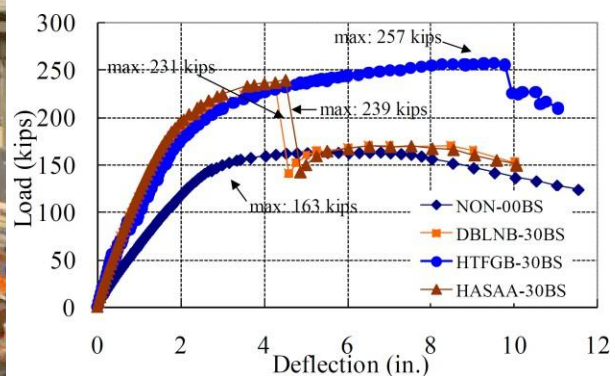
b) load-deflection curves
