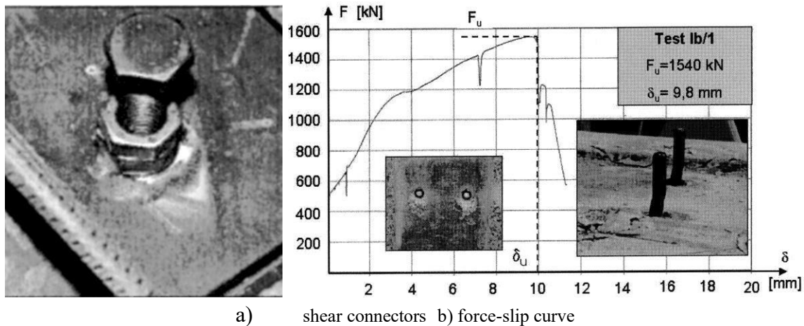
Fig. 2.8 Bolted shear connectors M20 [Sedlacek et al., 2003].
