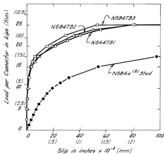
c) force-slip curves for 15.9 mm bolts
