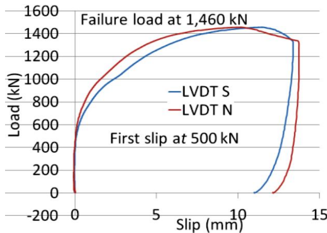
a) force-slip curve
